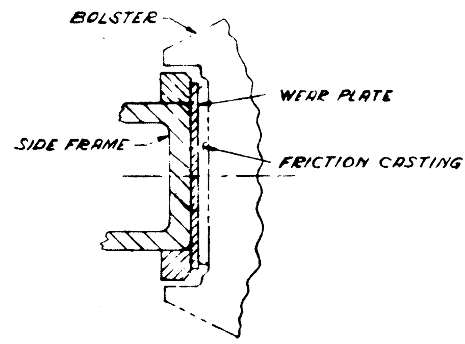
ENLARGED SECTION B-B
