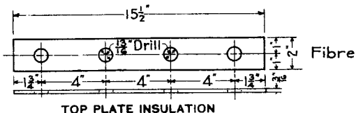
TOP PLATE INSULATION
