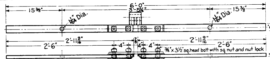
NO. 1 SWITCH ROD (Insulated)
