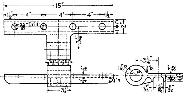
NON-INSULATED ROD BASKET
