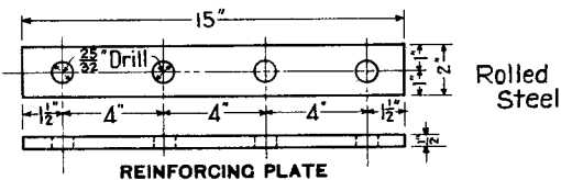
REINFORCING PLATE
