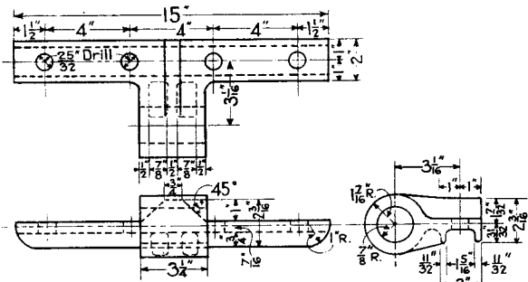
INSULATED ROD BASKET
