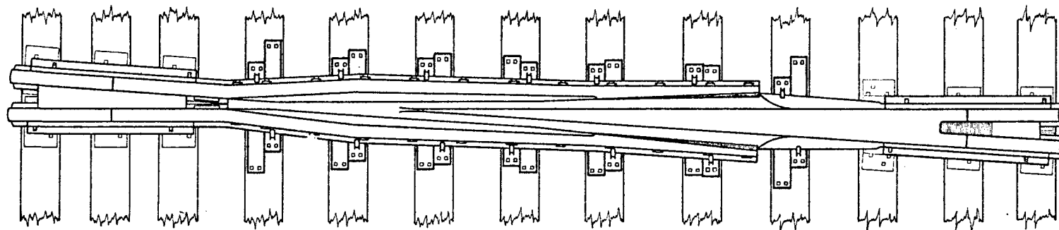
METHOD OF INSTALLING FROG TIE PLATES (No. 15 Frog - as drawn)
