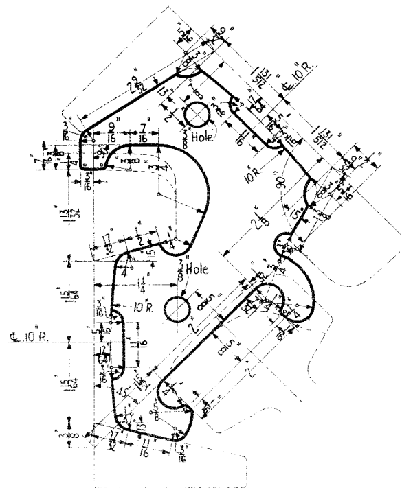
NO. 2 FIT GAUGE
