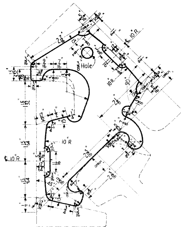
NO. 1 FIT GAUGE
