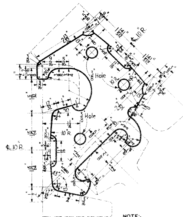
NO. 3 FIT GAUGE
