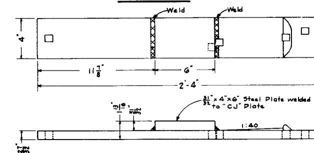
FT 20 FROG TIE PLATE MODIFIED
