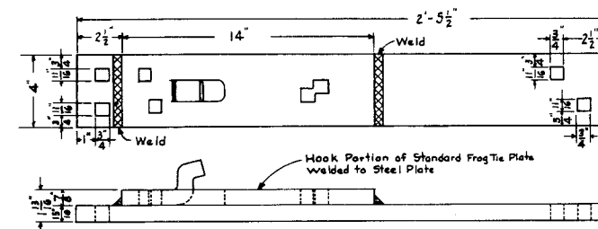
STANDARD FROG TIE PLATE MODIFIED
