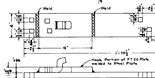
FT 20 FROG TIE PLATE MODIFIED
