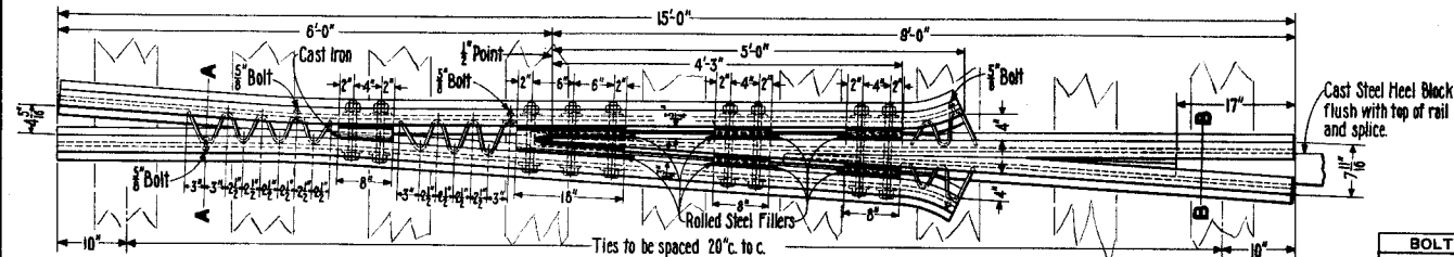
No. 15 FROG
