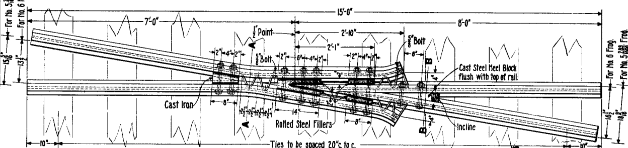
No. 5 289 / 1000 & 6 FROGS
