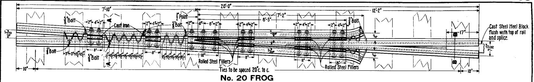
No. 20 FROG
