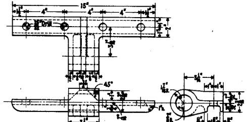
MALLEABLE IRON BASKET (for insulated rod)
