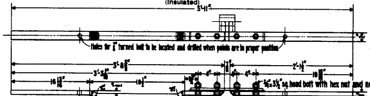
RODS NOS. 7 & 8 FOR SLIP CROSSING (Insulated)
