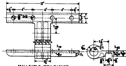
MALLEABLE IRON BASKET (for non-insulated rod)
