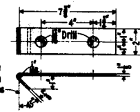
END OF ROD (showing bevel)
