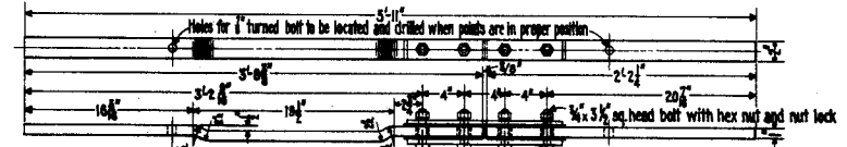
RODS NOS. 3, 4, 5 & 6 FOR SLIP CROSSING (Insulated)
