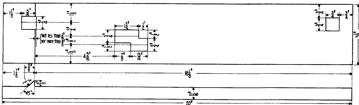
TYPE J PLATE
