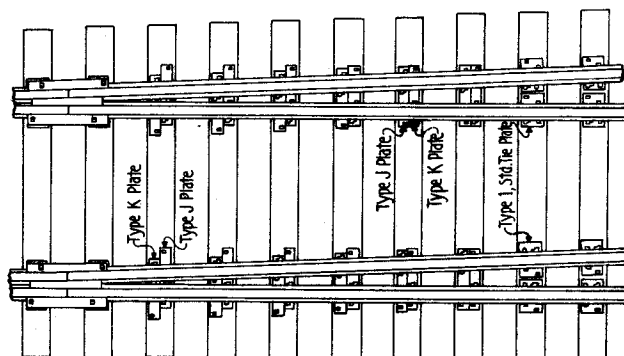
METHOD OF INSTALLING TWIN TIE PLATES
