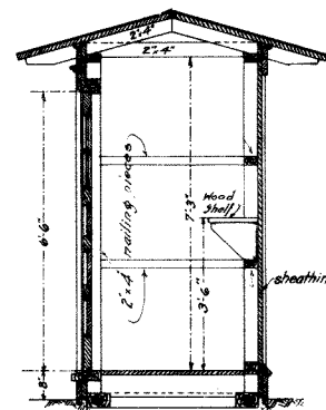
SECTION
