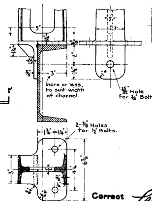
BASE STYLE D FOR USE ON CHANNEL
