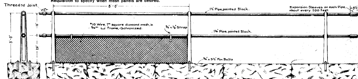
TWO PIPE RAILING
