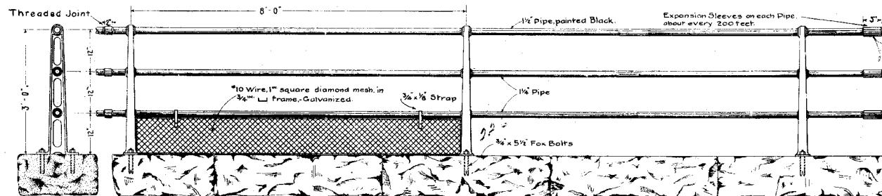
THREE PIPE RAILING
