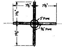
PLAN OF ANCHORING DEVICE
