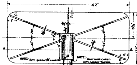
BACK VIEW
