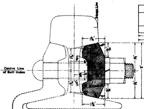
SECTION OF SPLICE BAR FOR 85 LBS. RAILS
