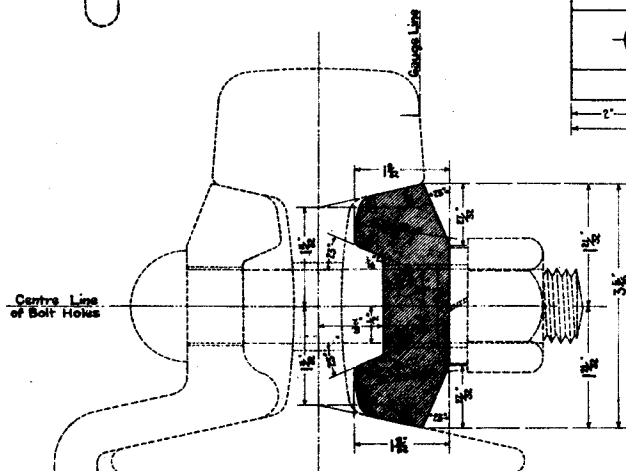
SECTION OF SPLICE BAR FOR 100 LBS. RAILS
