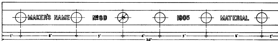
ELEVATION OF SPLICE BAR FOR 100 LBS. RAILS
