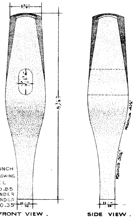
TRACK PUNCH .
