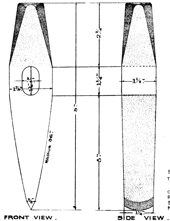
RAIL CUTTER .
