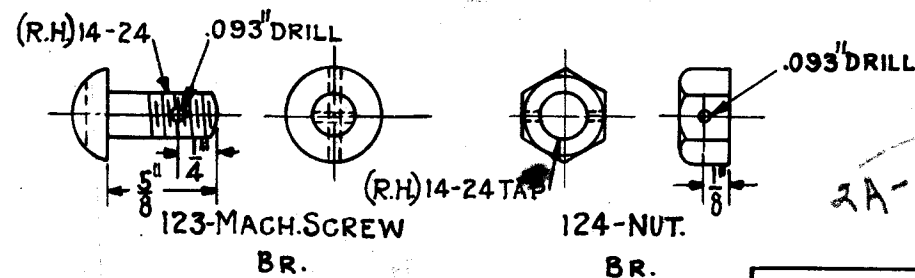
121- LOCKING AND SEALING DEVICE. COMPLETE AS SHOWN.
