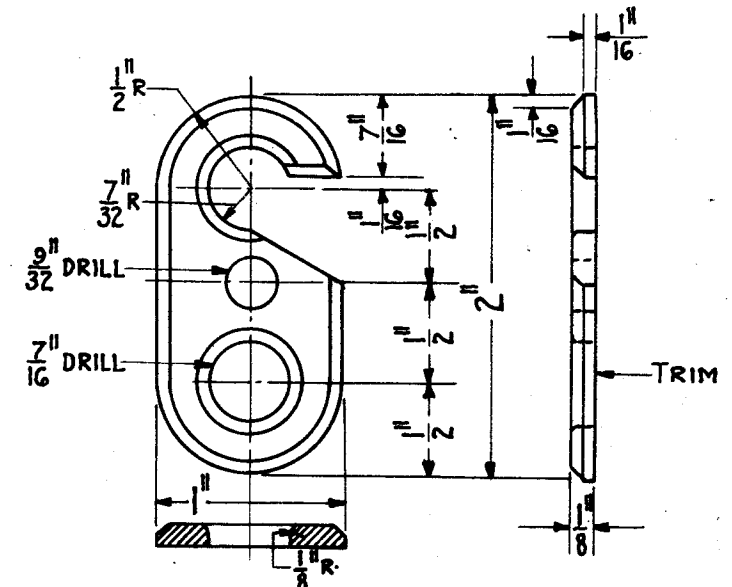
122- LOCK PLATE. CAST BRASS
