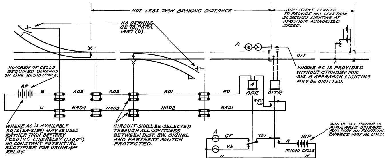
COLOR LIGHT DISTANT SWITCH SIGNAL FIG. C
