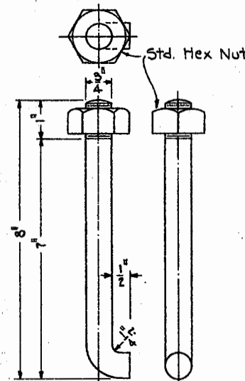
5464-HOOK BOLT G.I.
