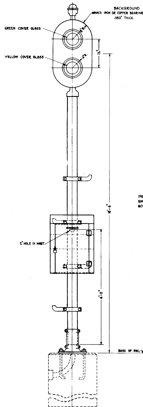
4701 - INDICATOR COMPLETE WITHOUT 4702.
