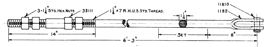
3358 - OPERATING ROD AS SHOWN - SET "A". 3359 - " " " " "B". 33510 - " " SET "A" WITHOUT 33111. 33511 - " " "B" " " F.S.
