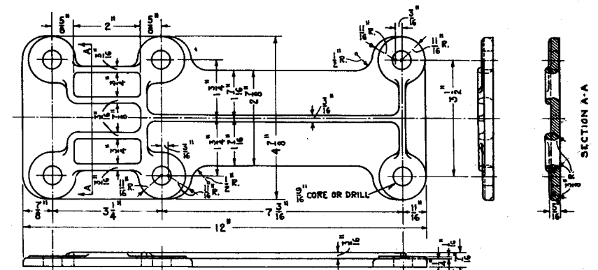
2564-COVER M.I. A.R.A. JUNE 1921
