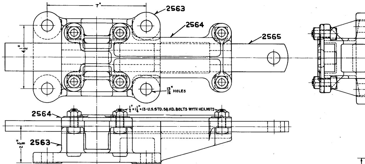
2561-PLUNGER LOCK COMPLETE. 2562- " " WITHOUT PLUNGER.
