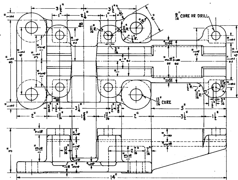
2563-STAND C.I. A.R.A. JUNE 1921
