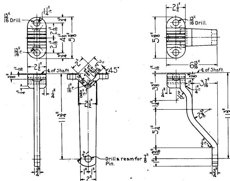
1544-STRAIGHT ARM.
