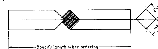
1543-SHAFT.
