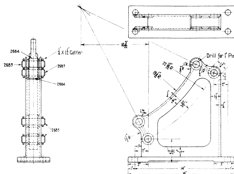
2683 - DEFLECTING STAND (CAST IRON)
