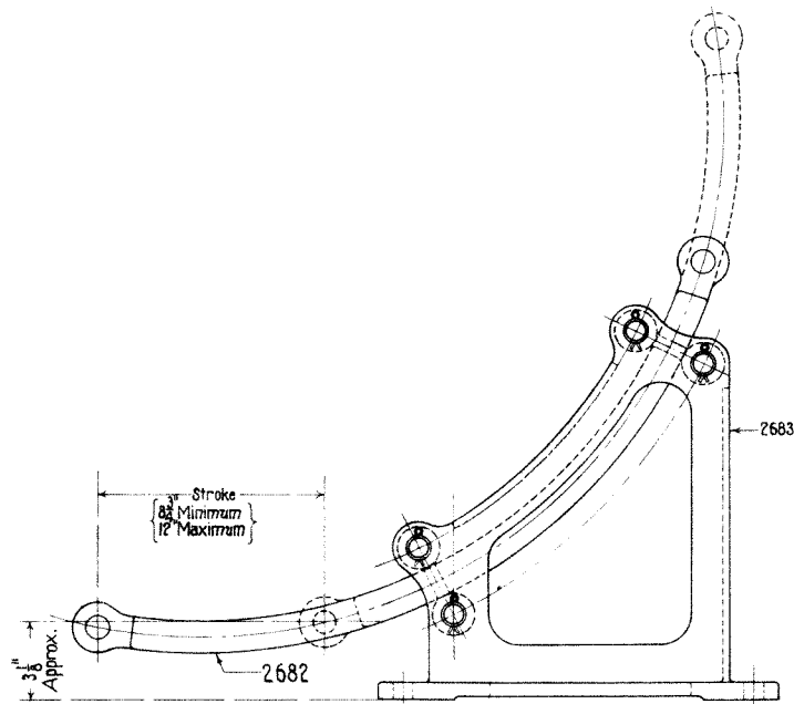
2681—VERTICAL DEFLECTING STAND COMPLETE
