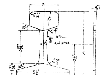
26516-FIBRE END POST For 125 lbs. Joint (A=6 1/2") 26517 .. .. . 130 .. .. . (A=6 3/4")
