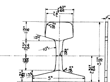
26511-FIBRE END POST For 100 lbs. Joint.
