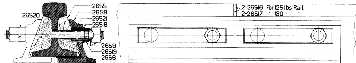
2652-4 HOLE INSULATING RAIL JOINT COMPLETE For 125 lbs. P. S. Rail. 2653-4 .. .. . 130 .. .. .
