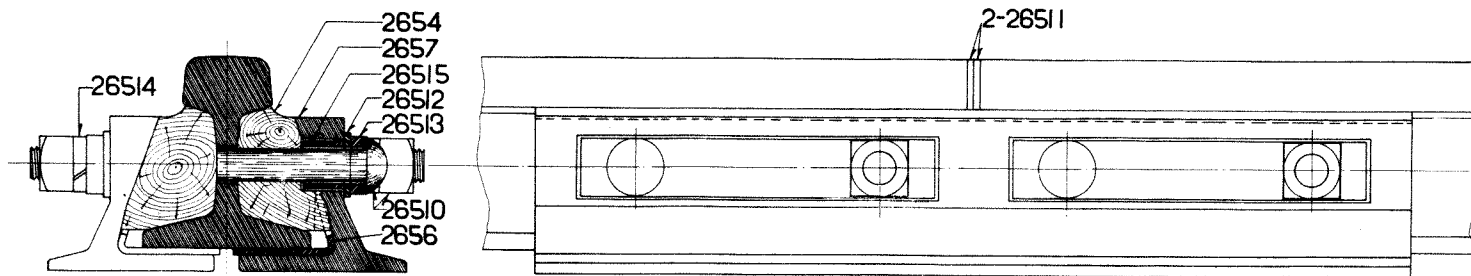
2651-4 HOLE INSULATING RAIL JOINT COMPLETE For 100 lbs. P. S. Rail.
