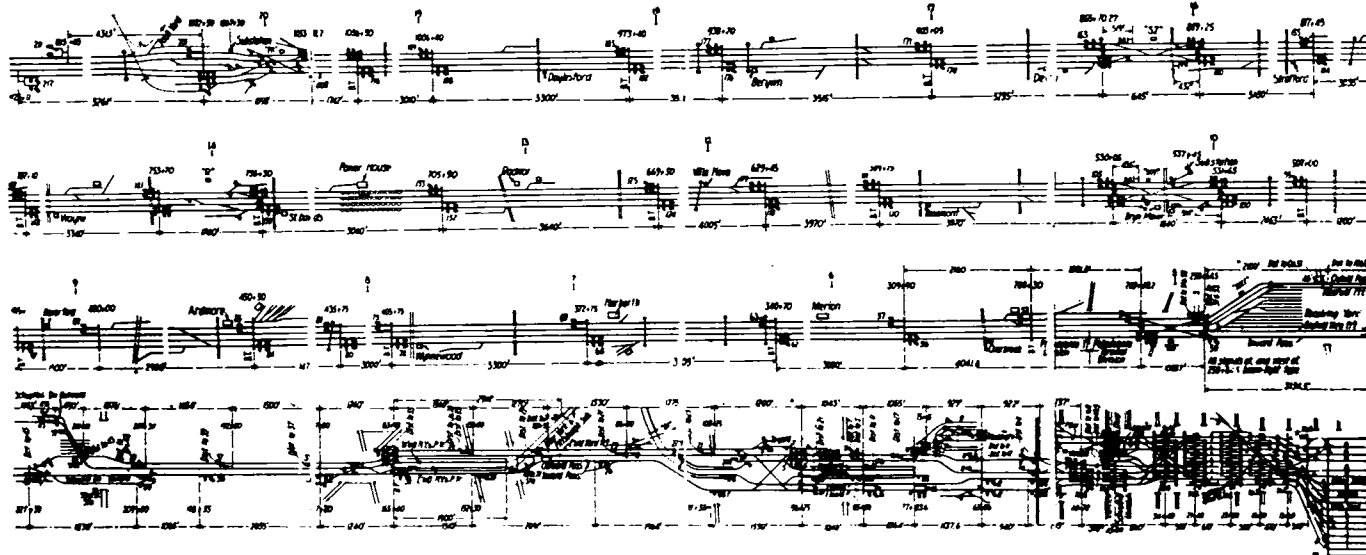
Track and Signal Layout of the Pennsylvania Railroad Between Broad Street Station, Philadelphia, and Paoli.
