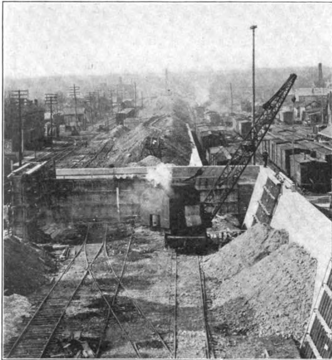
A View Through the Town During the Construction of the Retaining Walls, Showing Sectional Forms and Derrick Car for Handling Material
