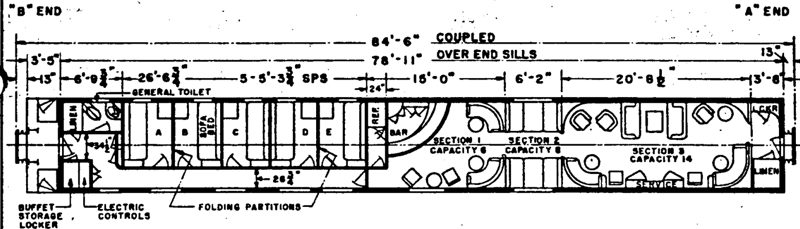
PASSENGER CAR CLASS PS5L 5 BEDROOM-BAR-LOUNGE PULLMAN BUILT -1938
