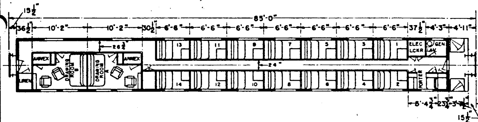
PASSENGER CAR CLASS PS 214 2 DRAWING ROOMS - 14 ROOMETTES ACF BUILT
