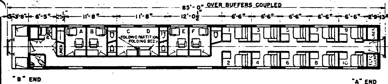
PASSENGER CAR CLASS PS106A 6 BEDROOMS, 10 ROOMETTES
