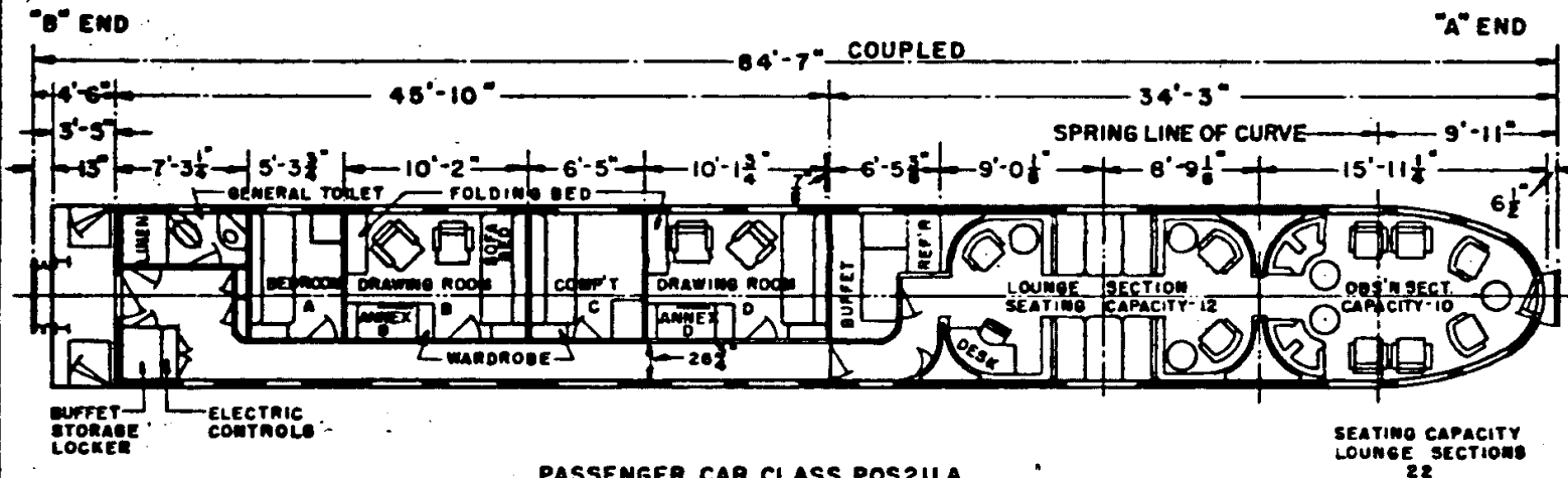
PASSENGER CAR CLASS POS211A 2 DRAWING ROOM-1 COMPARTMENT-1 BED ROOM-OBSERVATION PULLMAN BUILT - 1938
