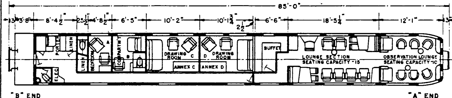
PASSENGER CAR CLASS POS 211 2 DRAWING ROOM - 1 COMPARTMENT - 1 DOUBLE BEDROOM - OBSERVATION PULLMAN BUILT
