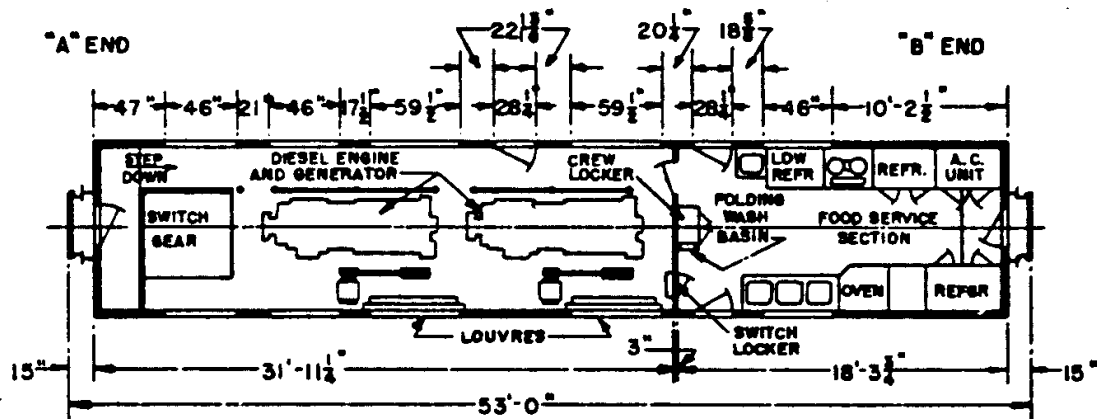
PASSENGER CAR CLASS HP53 POWER CAR WITH FOOD SERVICE SECTION TUBULAR TRAIN
