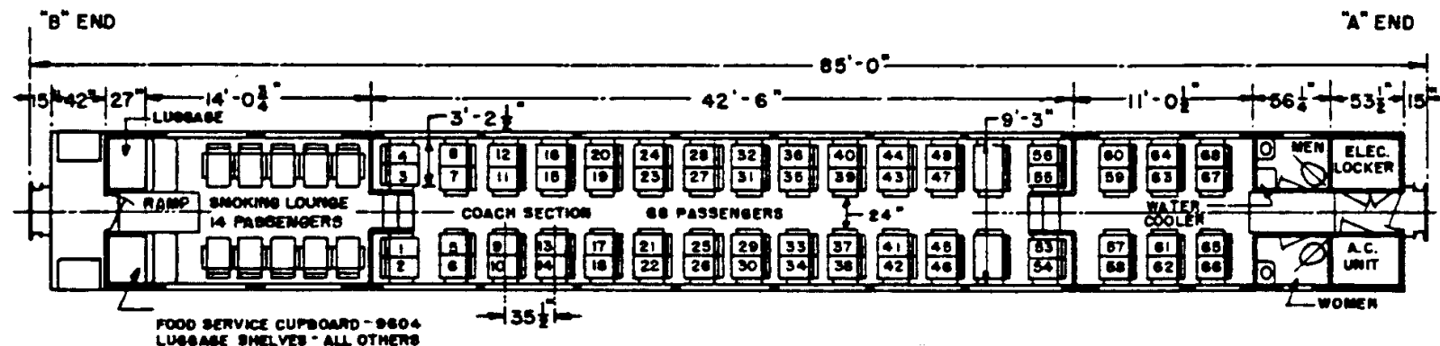
PASSENGER CAR CLASS P85K SEATING CAPACITY - 82 BUDD BUILT TUBULAR TRAIN
