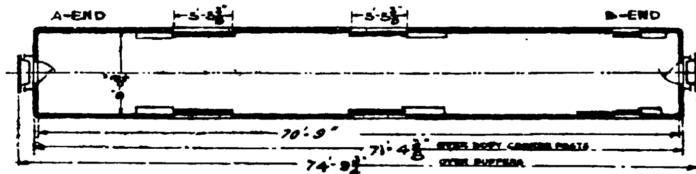
~ PASSENGER CARS CLASS B70B CONVERTED FROM BM70L
