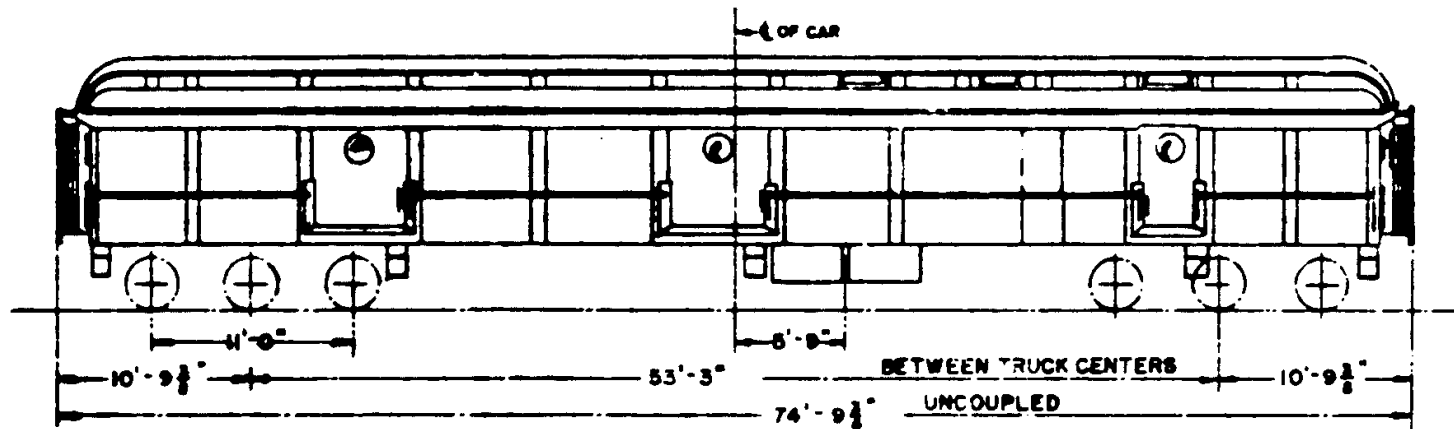
PASSENGER CAR CLASS 8708 CARS CONVERTED FROM CLASS BMTOKA
