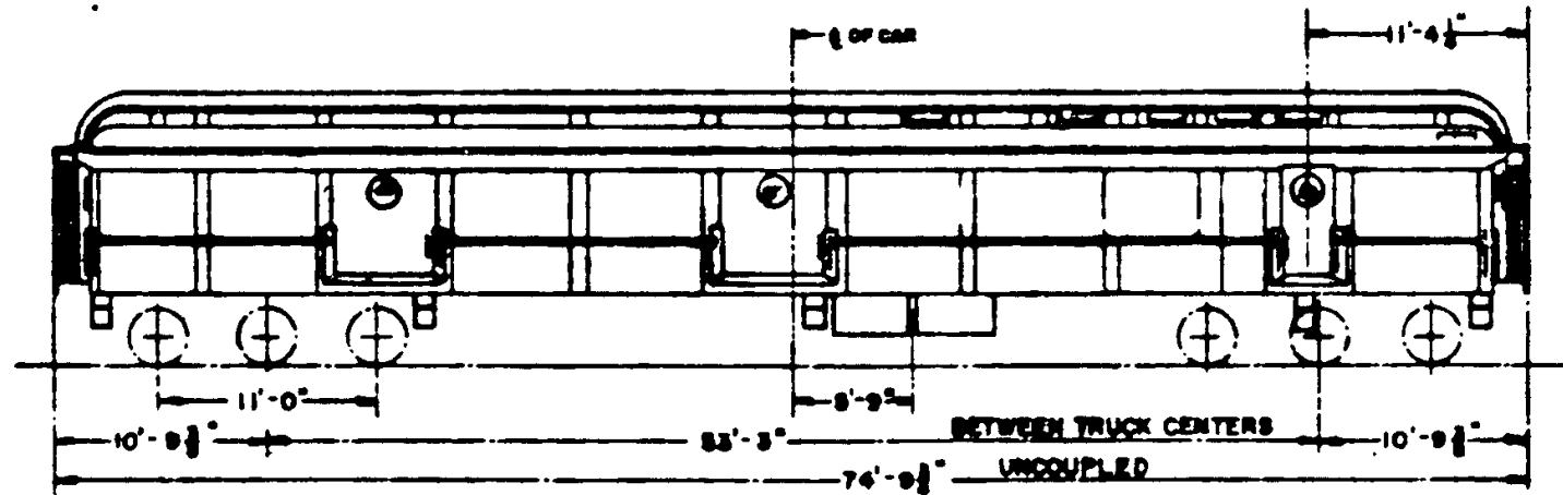
PASSENGER CAR CLASS CARS CONVERTED FROM CLASS BM70K CAR NO. 6144
