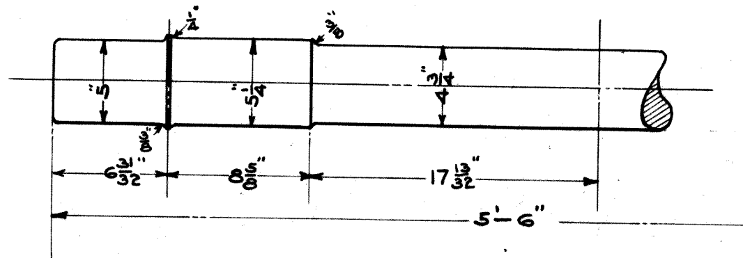
TRUCK AXLE FOR H3, H3A, H3B, LOCOMOTIVES. TRACING N2 11721. 10-15-96.
