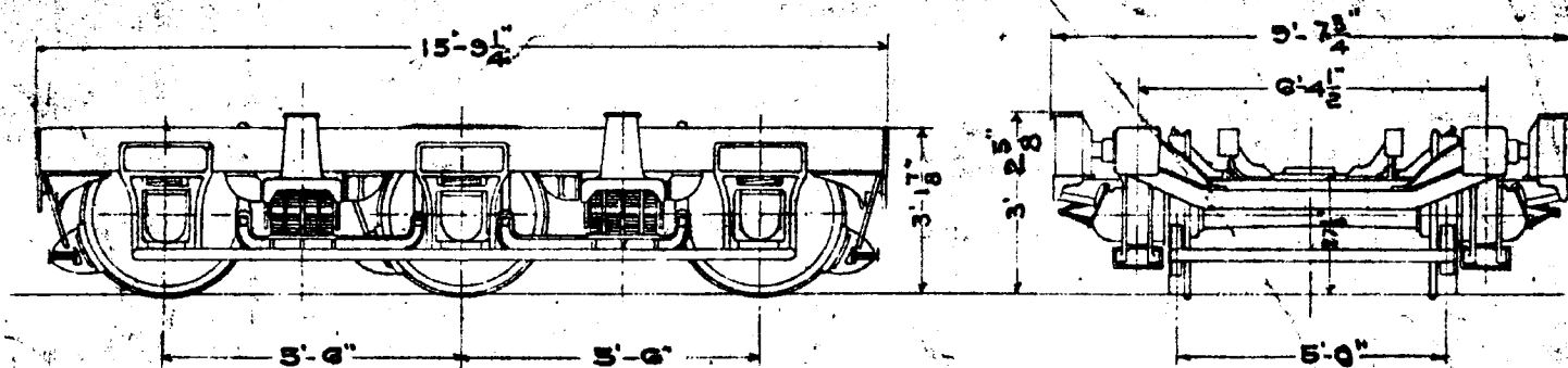
SIX WHEEL STEEL PASS. TRUCK NO. 1.
