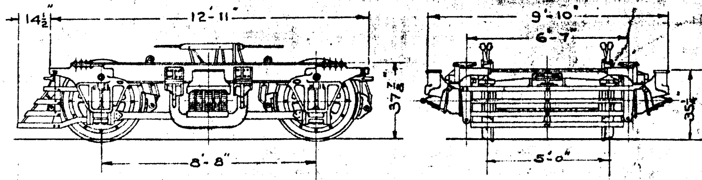
FOUR WHEEL STEEL PASS. MOTOR TRUCK No.8 M.
